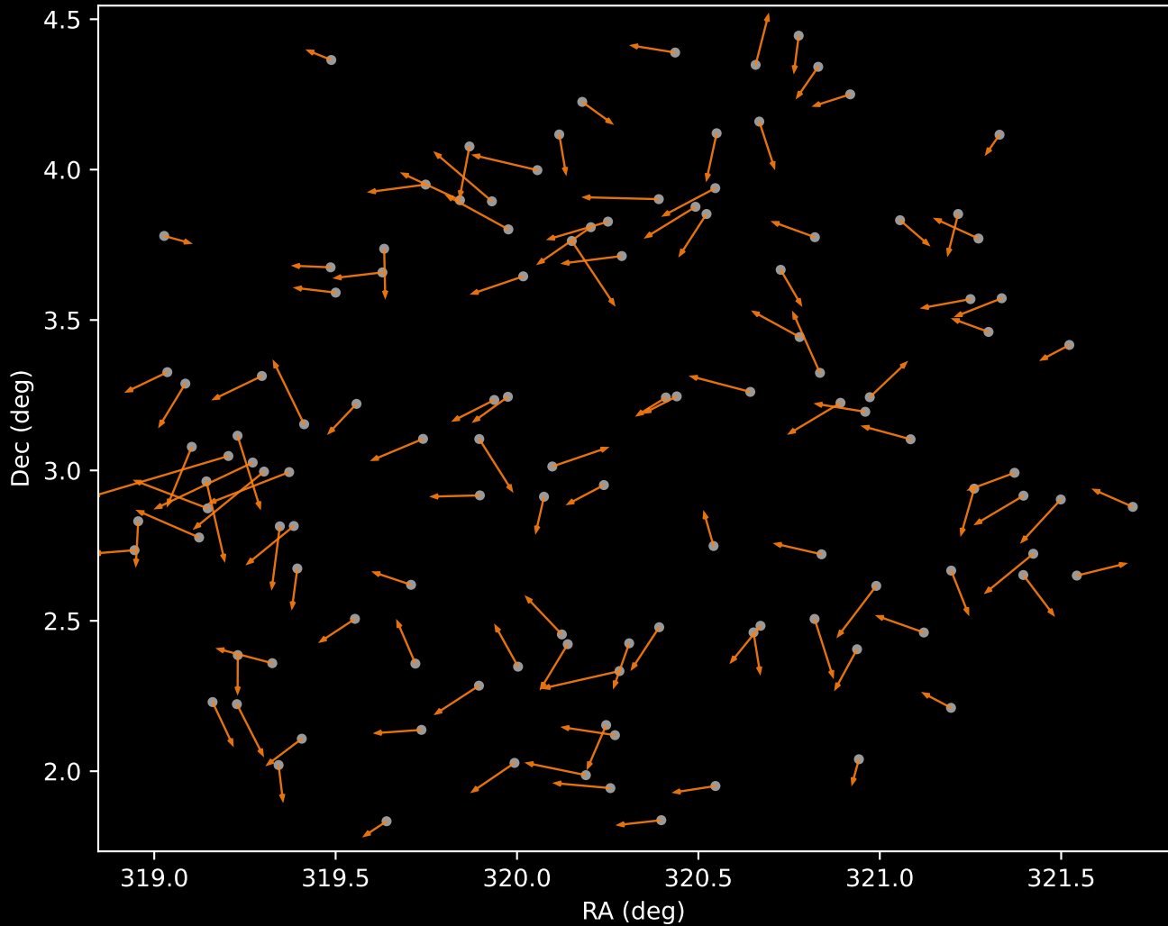
APOGEE DR17 Cluster 2 Proper Motion Vectors (n=120)
