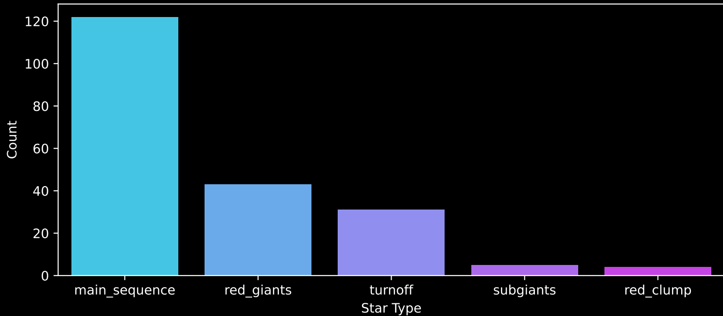
APOGEE DR17 Field: [355+55_MGA] Count plot of Star Type
