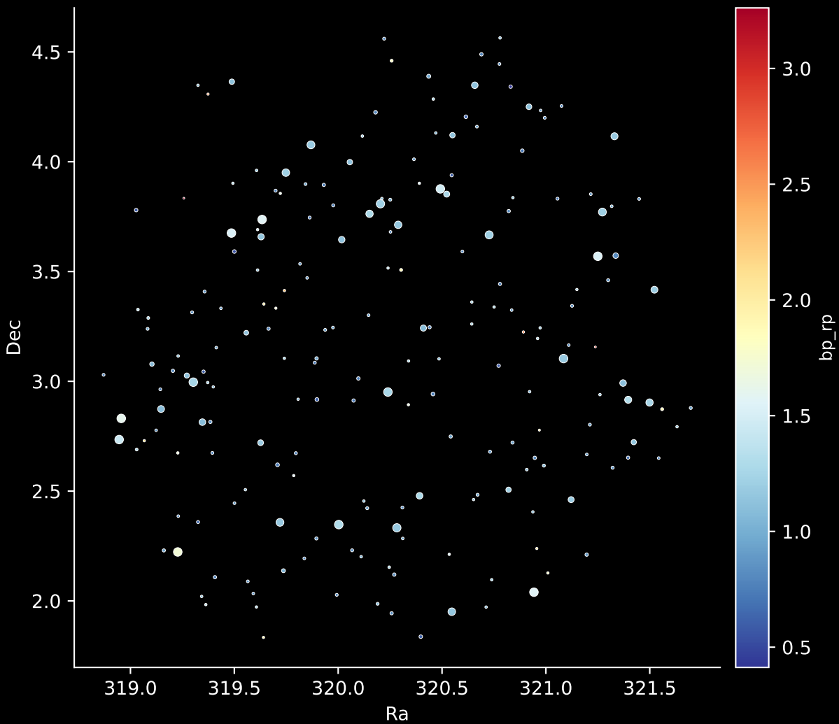
APOGEE DR17 Field: [355+55_MGA] Stars: 205
