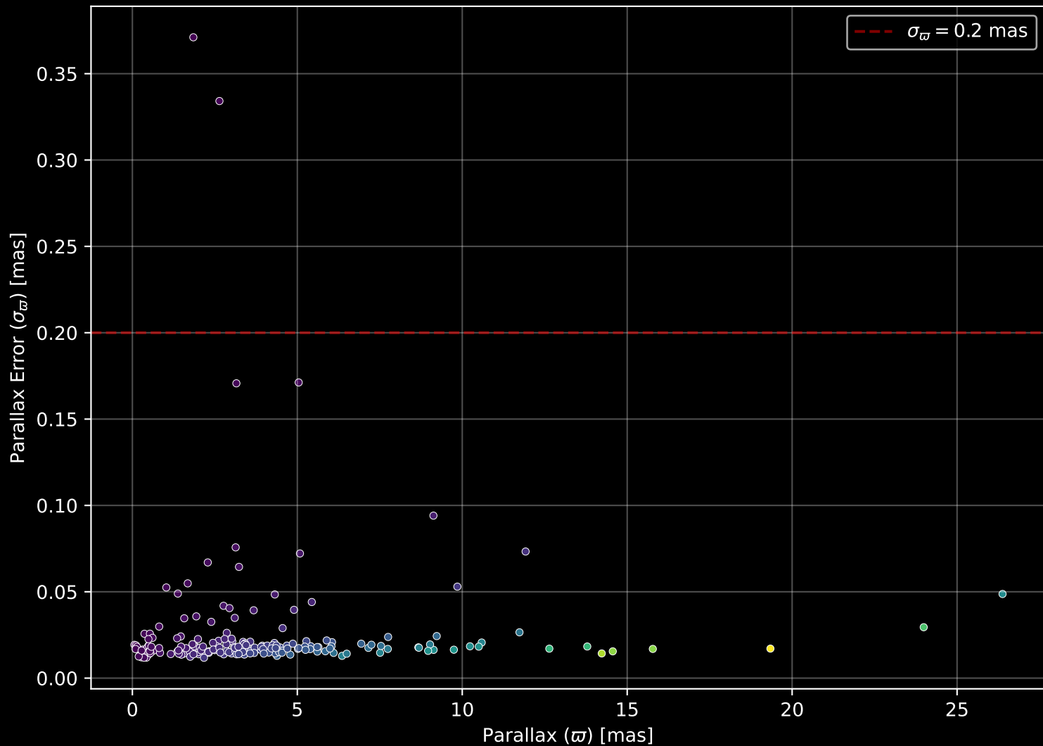
APOGEE DR17 Field: [355+55_MGA] Parallax Quality (n= 205)
