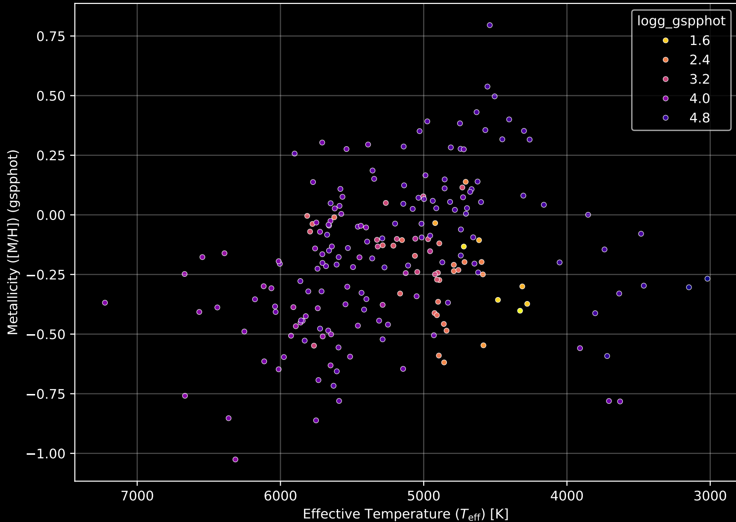
APOGEE DR17 Field: [355+55_MGA] Stellar Population Parameters (n= 205)
