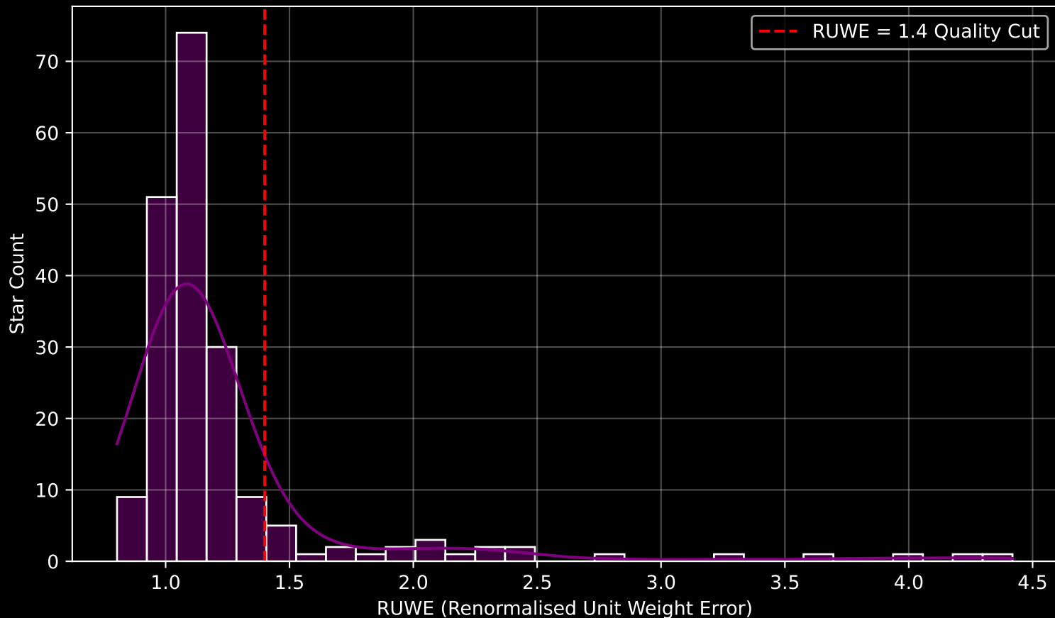
GAPOGEE DR17 Field [355+55_MGA] RUWE Distribution (n= 198)
