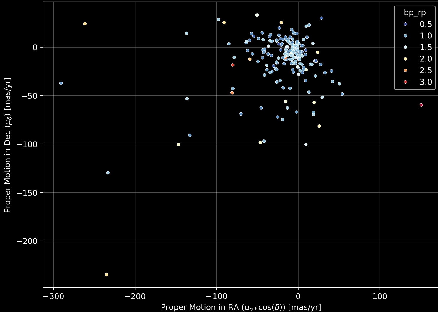
APOGEE DR17 Field: [355+55_MGA] Proper Motion Diagram (n= 205)
