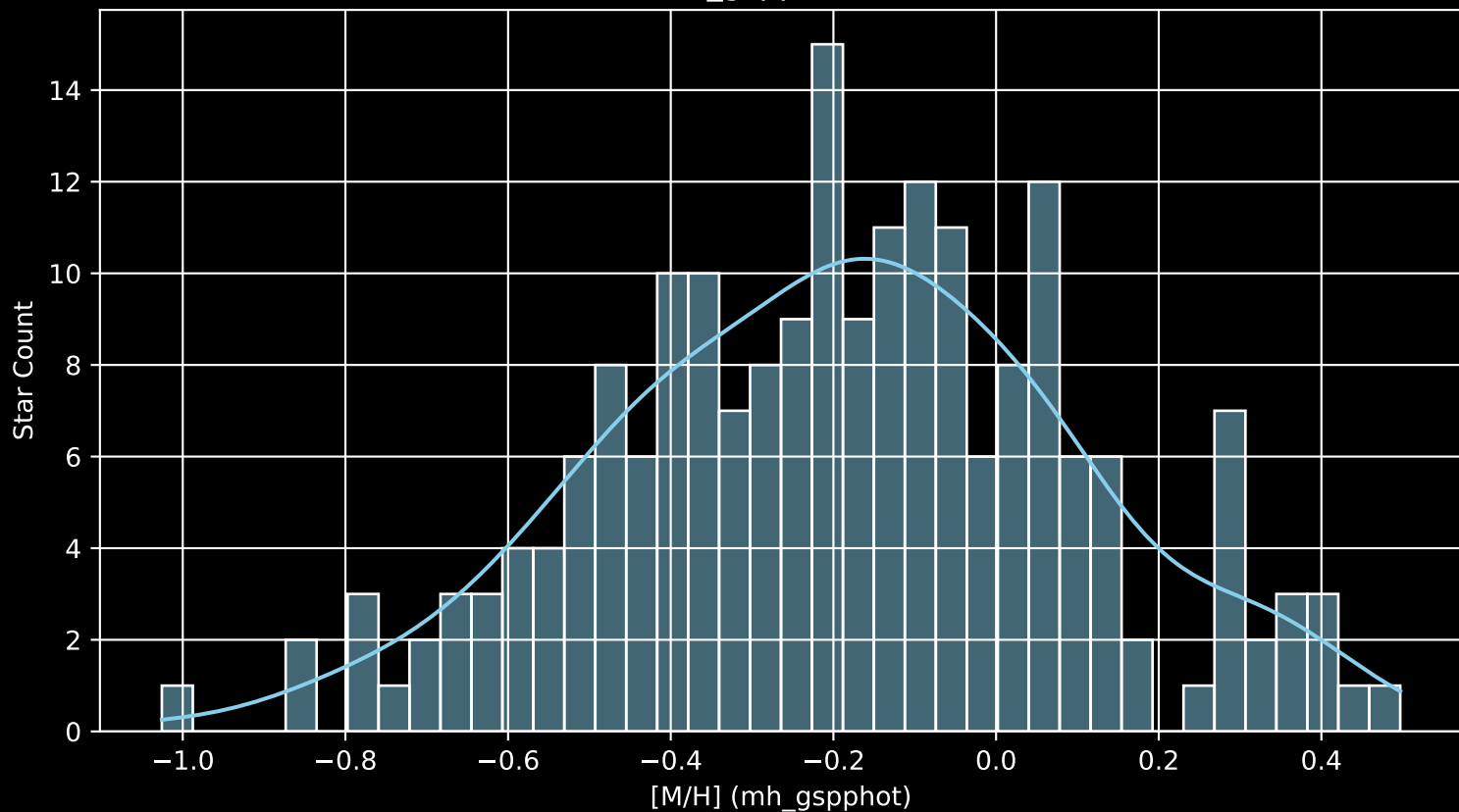
APOGEE DR17 Field: [355+55_MGA [M/H] (mh_gspphot) (n= 203)
